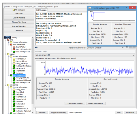
Robust Cyber Simulation and Training Tool
